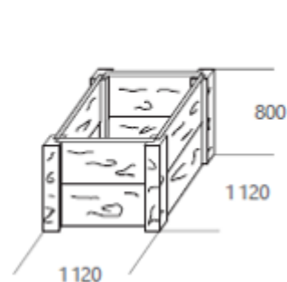
Visoka greda 112 x 112 x 80
